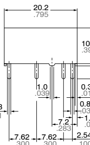
2 coil latching
