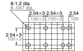
PC board pattern (Copper-side view) Single side stable 2 coil latching
