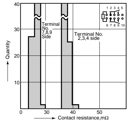
11. Distribution of contact resistance
