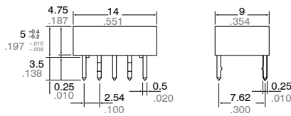
Self-clinching terminal
