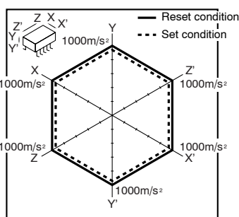
12.-(2) Malfunctional shock (latching) Tested sample: TQ2SA-L2-12V, 6 pcs.
