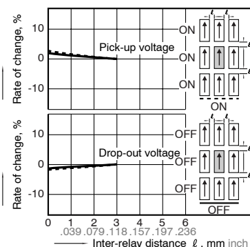
13.-(3) Influence of adjacent mounting Tested sample: TQ2SA-12V, 6 pcs.
