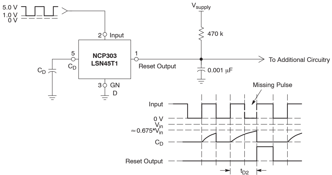
Figure 40. Missing Pulse Detector or Frequency Detector
