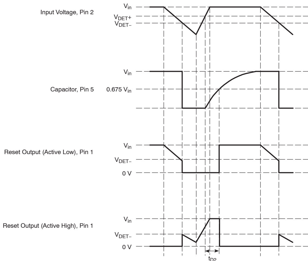
Figure 37. Timing Waveforms
