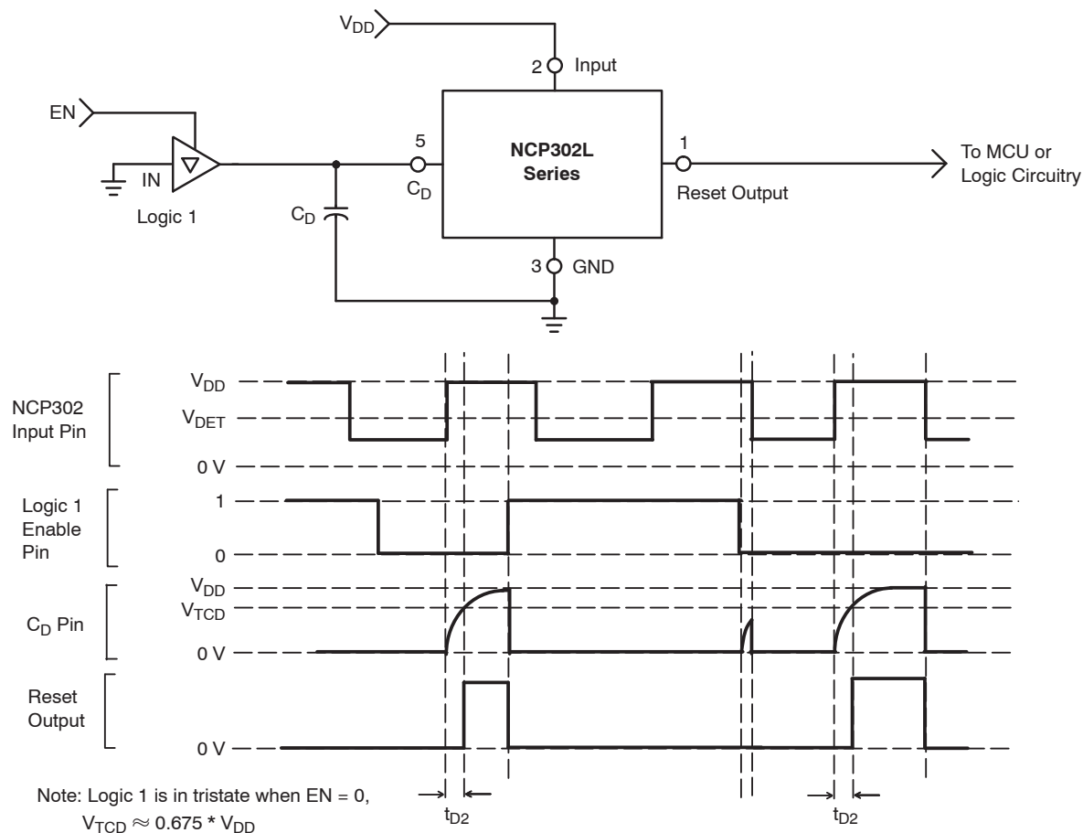
Figure 45. Undervoltage Detection with Independent Reset Signal Control
