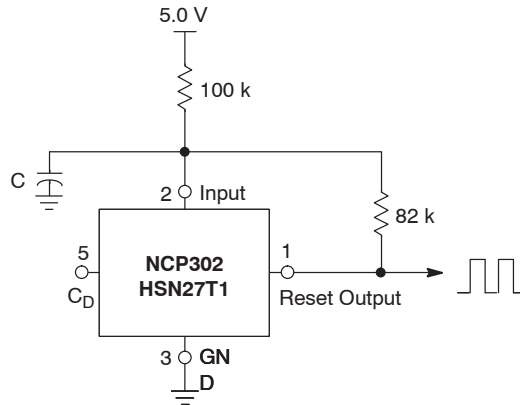
Figure 42. Simple Clock Oscillator
