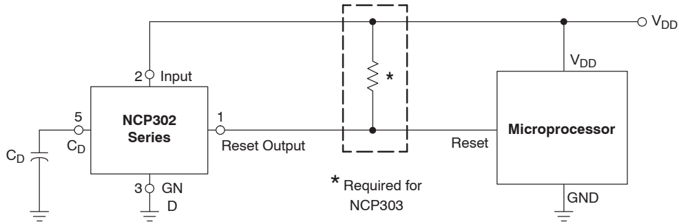
Figure 38. Microprocessor Reset Circuit
