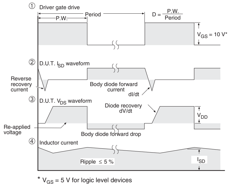
Fig. 11 - For N-Channel
