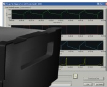
C5 - Software
